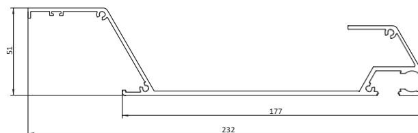
plochá lamela - led
